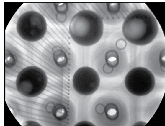
X-ray Image of BGA Voids as seen through a micro-chip with the Ultra-Compact.
